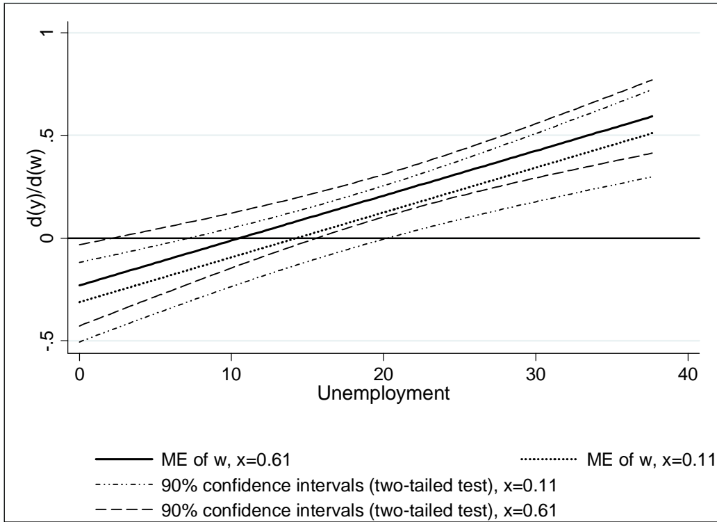
Figure 3A. Marginal effects of social capital as a function of unemployment at 25 th and 75 th percentiles of immigration
