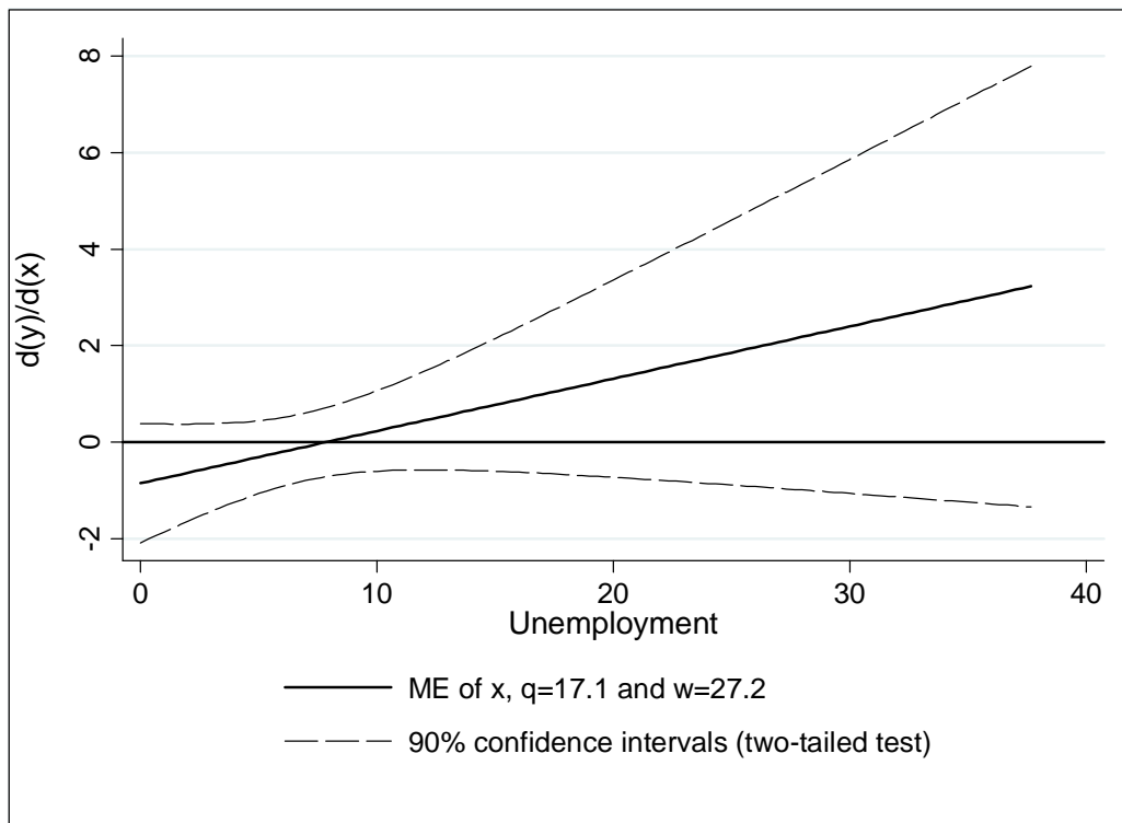
Figure 1B. Marginal effects of immigration as function unemployment of at median values of fiscal redistribution and social capital
