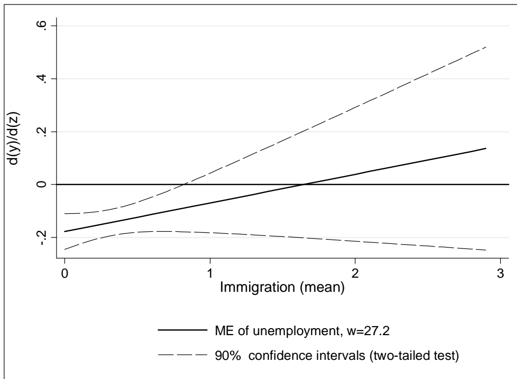
Figure 1A. Marginal effects of unemployment as a function of immigration at median value of social capital
