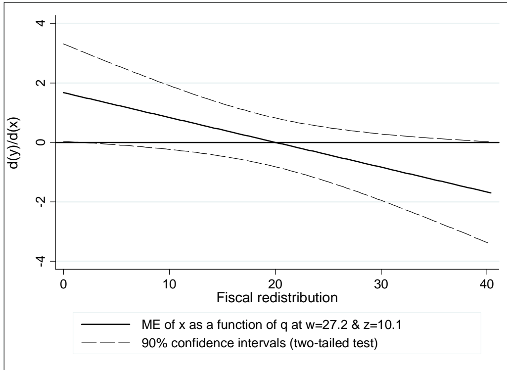
Figure 2B. Marginal effects of immigration as a function of fiscal redistribution at median values of social capital and unemployment
