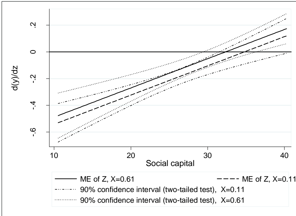
Figure 3B. Marginal effects of unemployment as a function of social capital for high and low values of immigration
