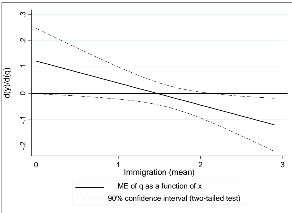
Figure 2A. Marginal effects of fiscal redistribution as a function of immigration
