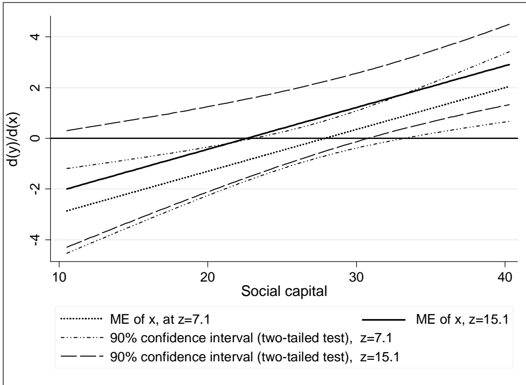
Figure 3C. Marginal effects of immigration as a function of social capital at 25th and 75th percentiles of unemployment and median fiscal redistribution
